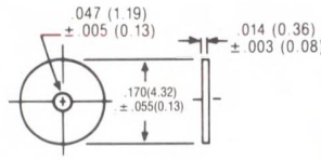
MOUNTING PAD
